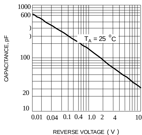
Fig. 4-TYPICAL JUNCTION CAPACITANCE
