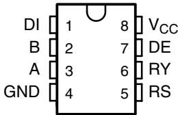
SN75119 . . . D OR P PACKAGE (TOP VIEW)
