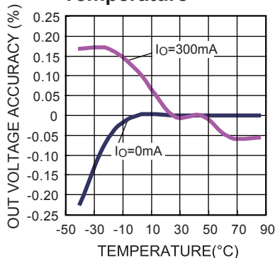
Out2 Voltage Accuracy vs. Temperature
