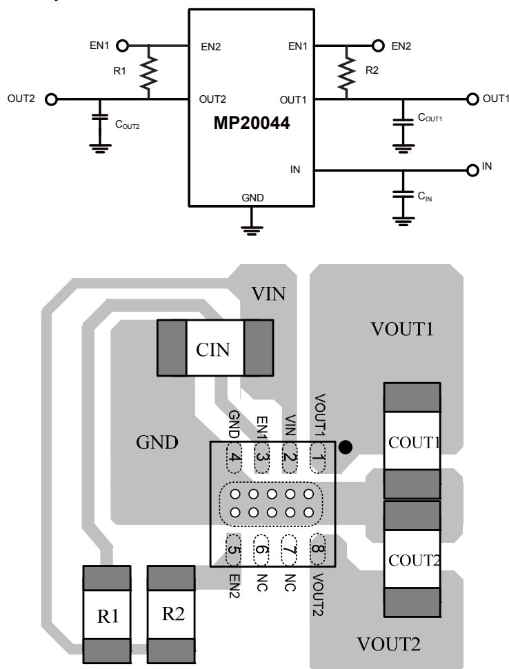
Top Layer Figure 5—PCB Layout
