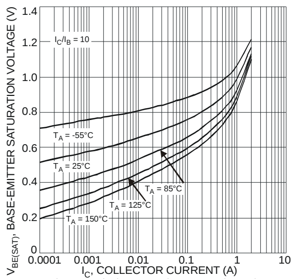
Fig. 11 Typical Base-Emitter Saturation Voltage vs. Collector Current
