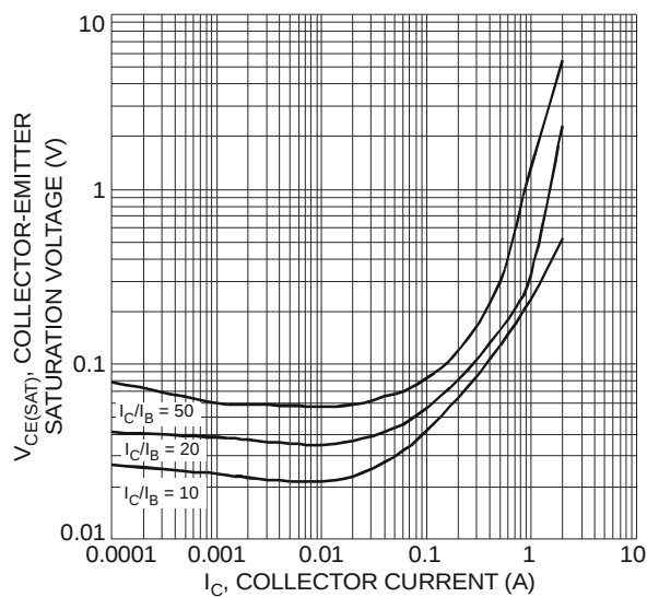
Fig. 9 Typical Collector-Emitter Saturation Voltage vs. Collector Current
