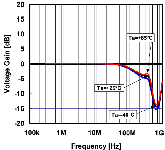
Voltage Gain vs. Frequency (correlation with T_a )
