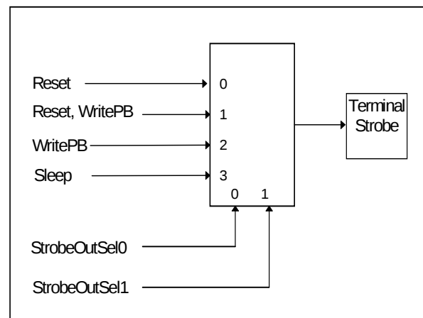
Figure 32 . Strobe Output
