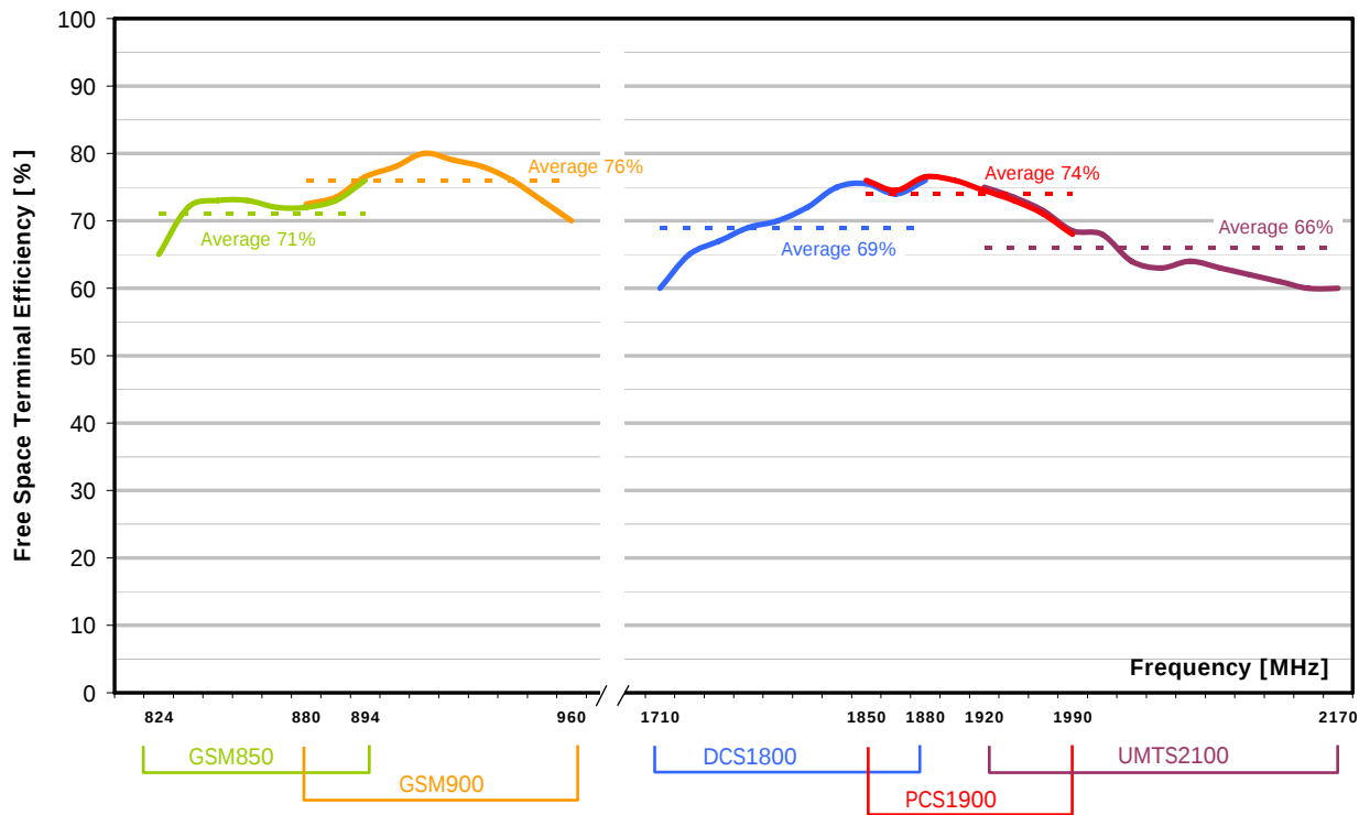
Reflexus efficiency in free space
