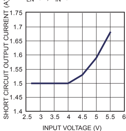
Short Circuit Output Current vs. Input Voltage
