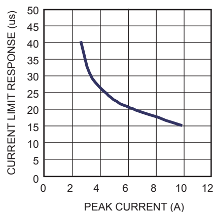
Current Limit Response Time vs. Peak Current
