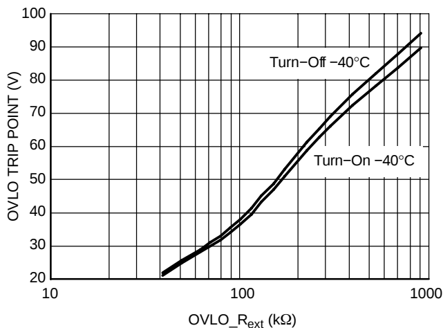
Figure 6. OVLO Adjustment, T J = -40°C
