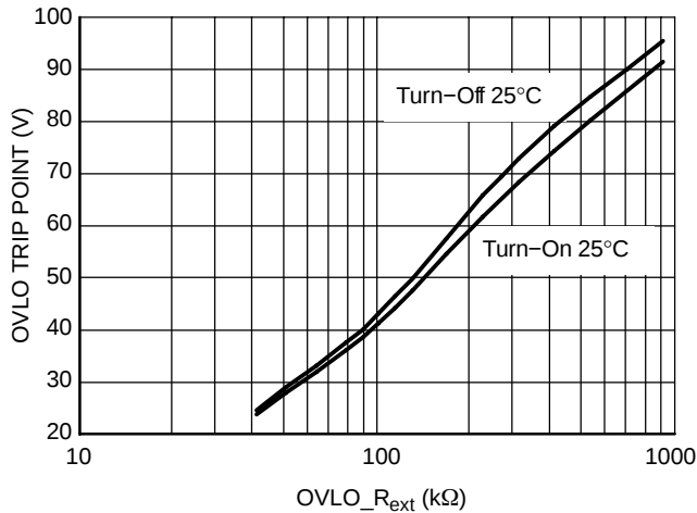
Figure 4. OVLO Adjustment, T J = 25°C
