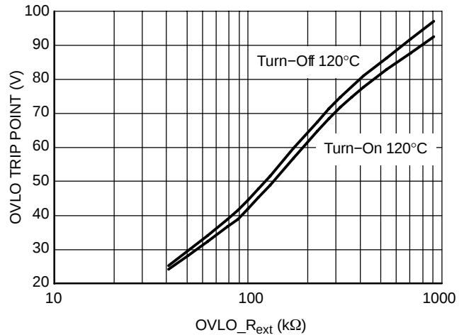
Figure 5. OVLO Adjustment, T J = 120°C
