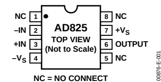
Figure 4. 8-Lead SOIC
