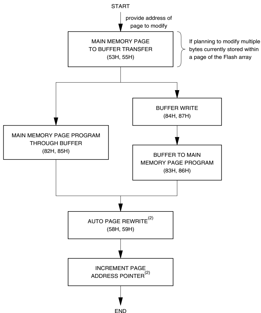
Figure 15-2. Algorithm for Randomly Modifying Data
