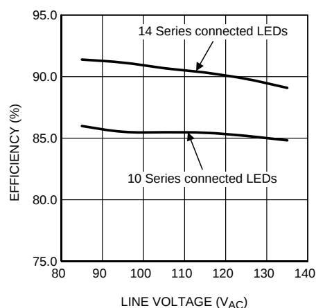
Efficiency vs Line Voltage
