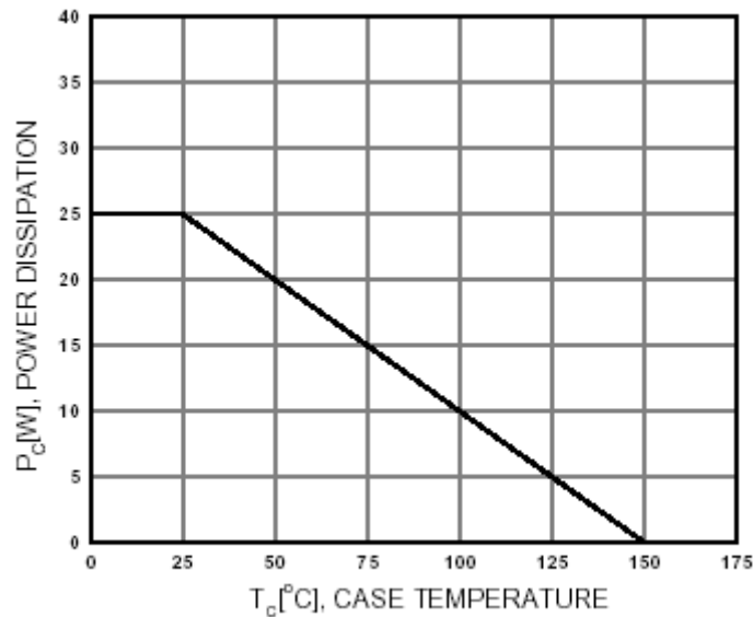
Fig.7 Power Derating
