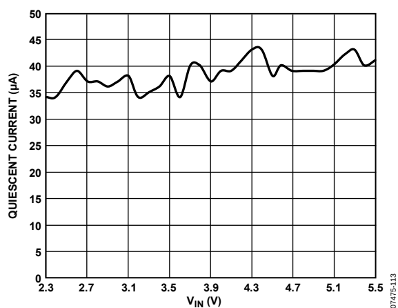
Figure 14. Quiescent Current vs. Input Voltage ( V_{OUT} = 3.3 V)
