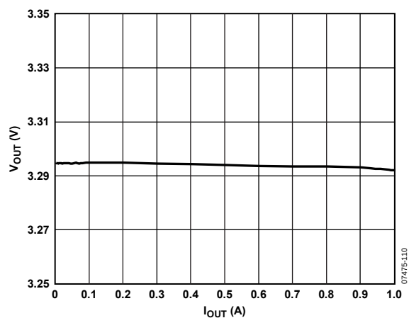
Figure 12. Load Regulation ( V_{IN} = 3.6 V, V_{OUT} = 3.3 V)
