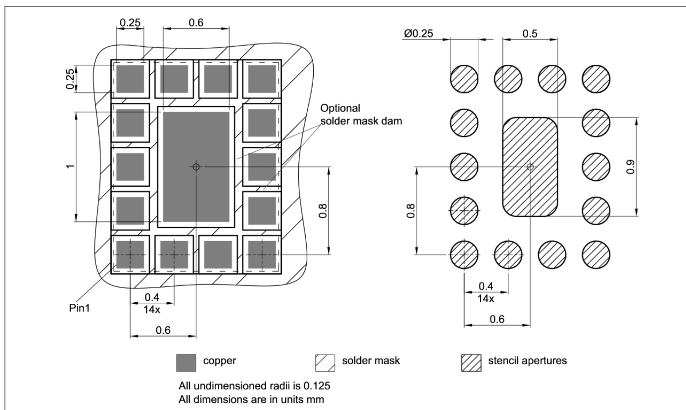
Figure 5: Footprint Recommendation
