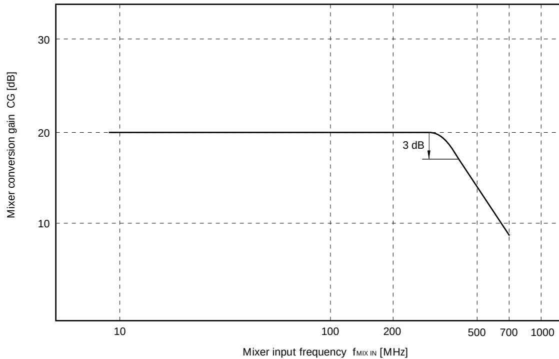
Figure 4-3. Mixer Conversion Gain vs. Mixer Input Frequency ( V_{\text{MIX IN}} = -30 dBm, V_{\text{OSC IN}} = -15 dBm, f_{\text{OSC IN}} = f_{\text{MIX IN}} - f_{\text{MIX OUT}} , f_{\text{MIX OUT}} = 455 kHz)
