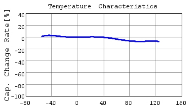
■ GCD216R71H392KA01 C-Temp. capchange, DC0.0V,
