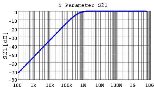
■ GCD216R71H392KA01 S21 DC0V, 25degC
