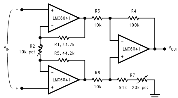
Figure 39. Instrumentation Amplifier
