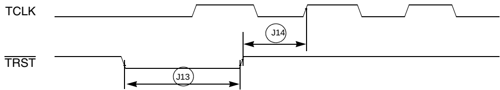
Figure 31. \overline{\text{TRST}} Timing
