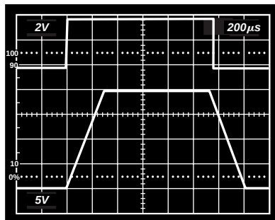
Figure 2. Small-Signal Transient Response
