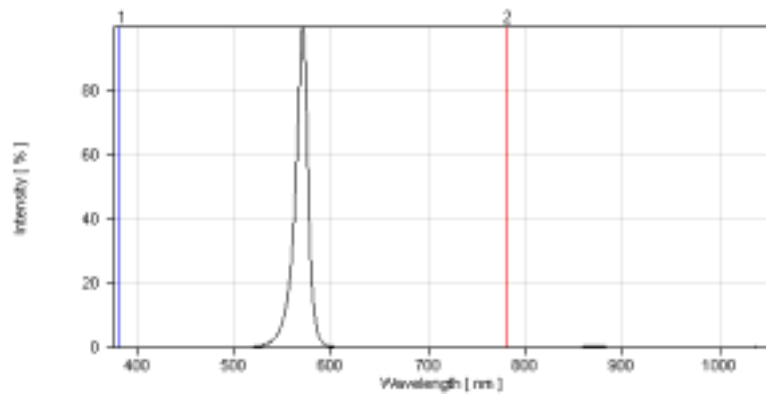
Fig.2 Yellow Green Relative Intensity vs. Wavelength
