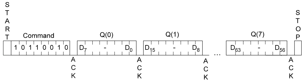
Figure 10. Initiatize Authentication
