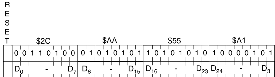
Figure 8. Answer-to-reset Values
