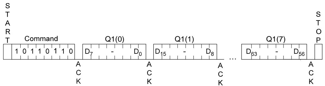
Figure 11. Verify Authentication
