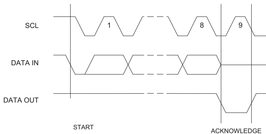
Figure 6-6. Output Acknowledge
