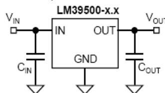
Fig 1. Capacitor Requirements
