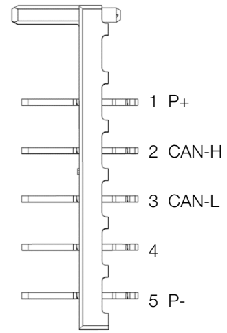
Device Counterpart for CAN-Bus
