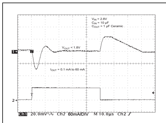
FIGURE 2-22: Load Transient Response.
