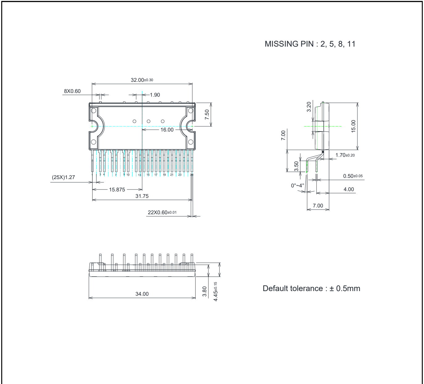
Figure 18 IM393-S6F
