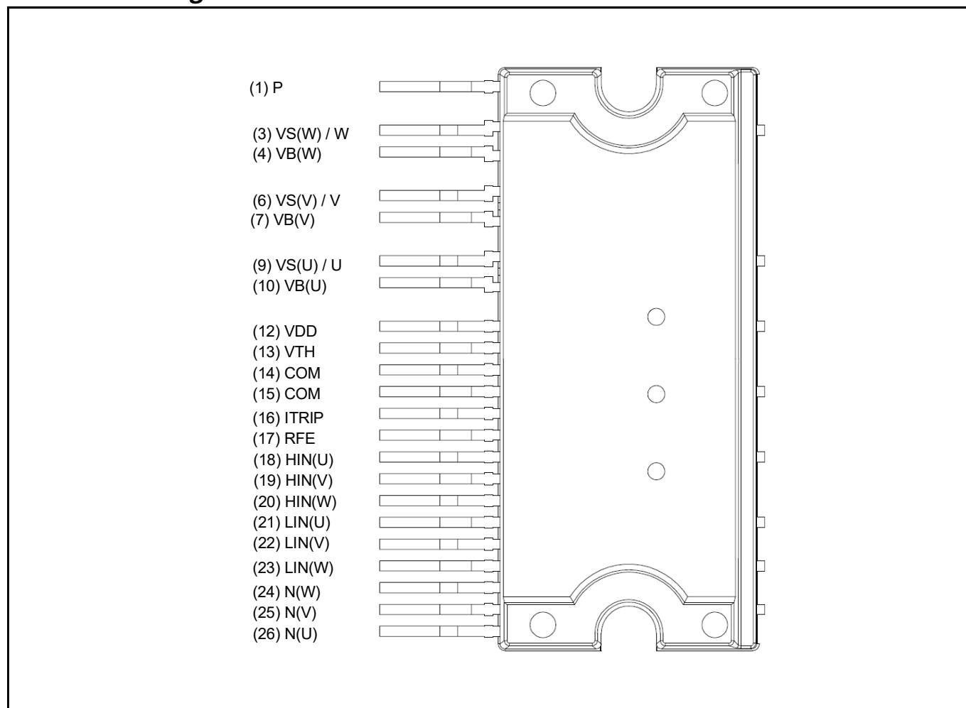
Figure 2 Pin configuration
