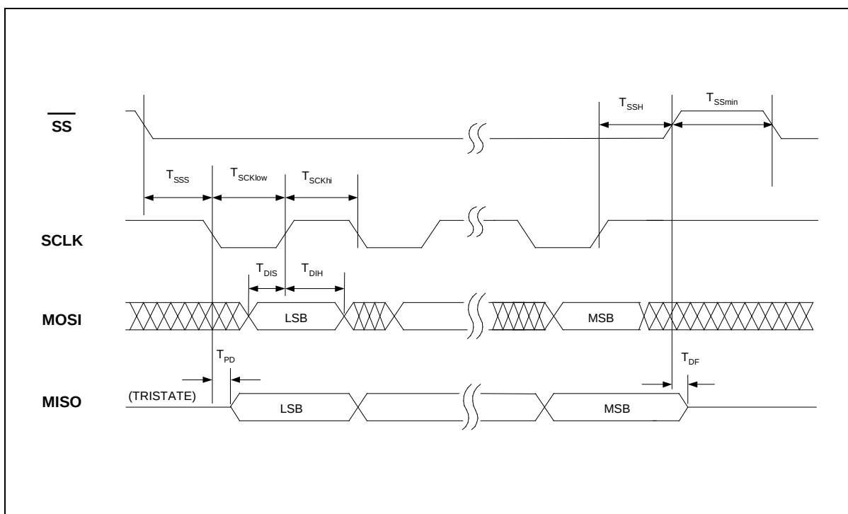
Figure 12.8: SPI Operation
