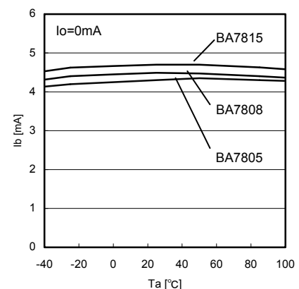
Fig.23 T_a - I_b
