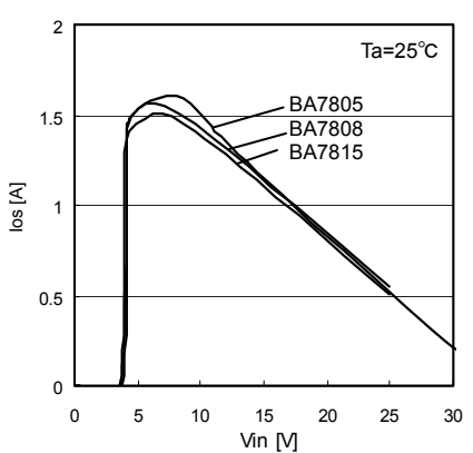
Fig.20 Short - Circuit Output Current
