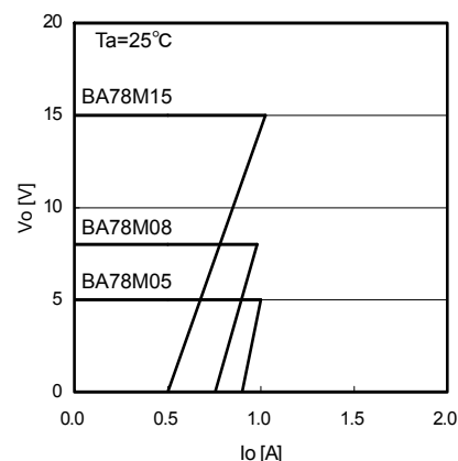
Fig.5 Load Regulation
