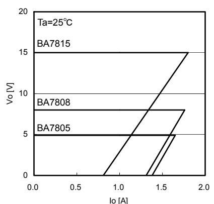
Fig.17 Load Regulation
