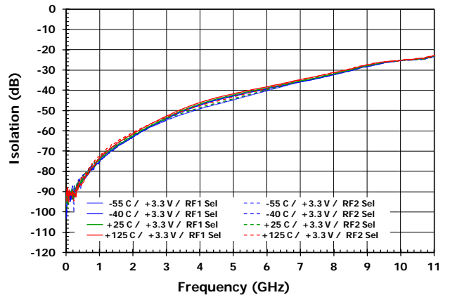
Figure 13. Isolation vs. Voltage [RF1 → RF2]
