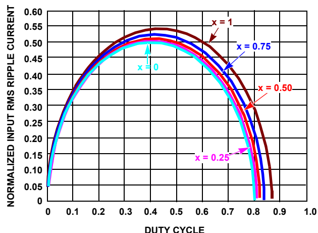
FIGURE 5. NORMALIZED RMS INPUT CURRENT FOR x = 0.8
