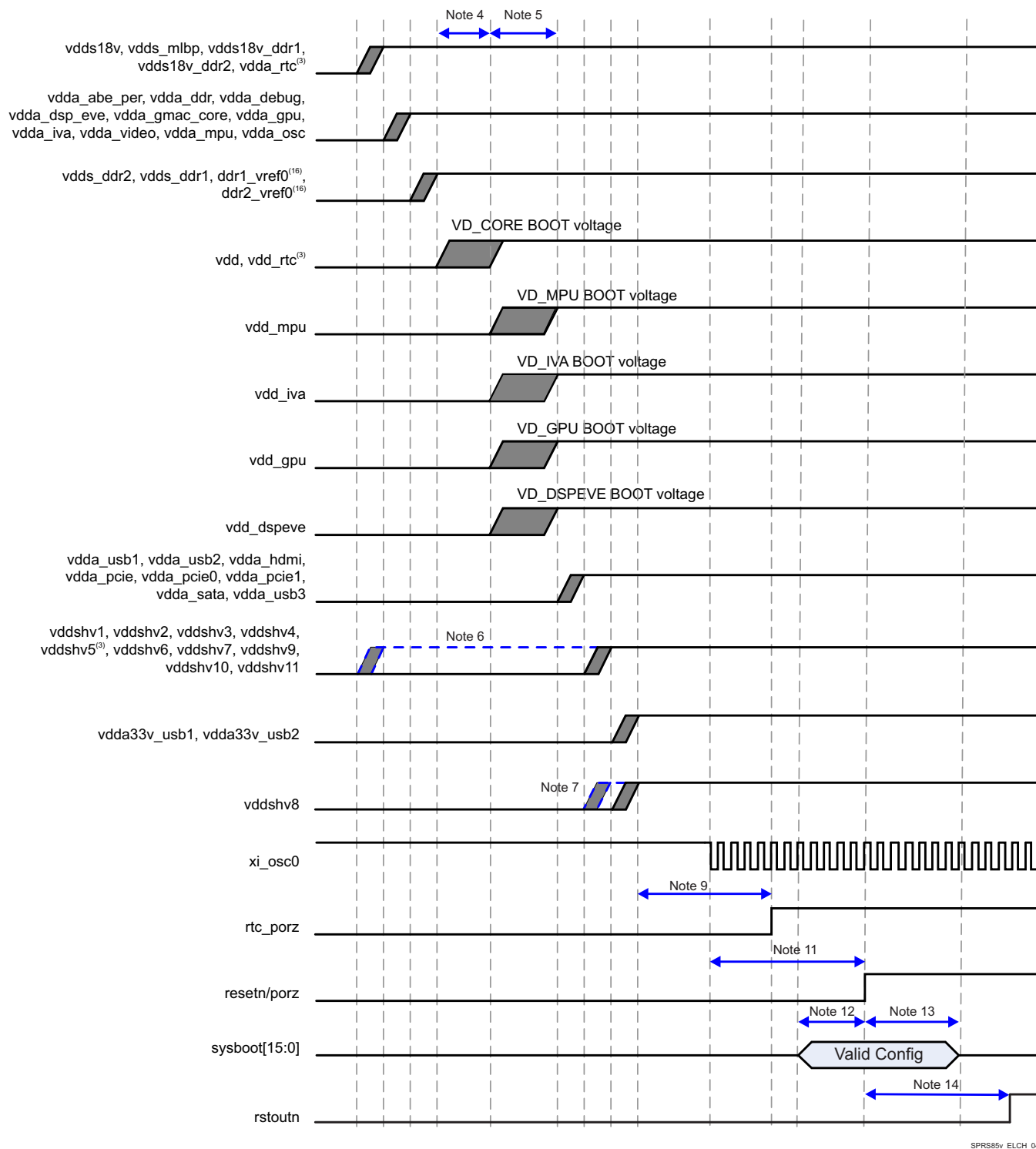
图 5-2. Power-Up Sequencing
