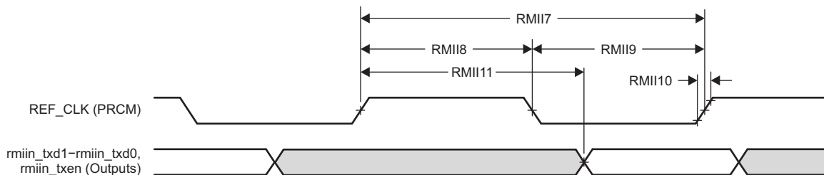
图 7-57. GMAC Transmit Interface Timing RMIIIn Operation
