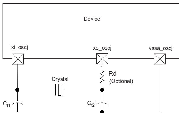
图 8-33. Grounding Scheme for High-Frequency Clock
