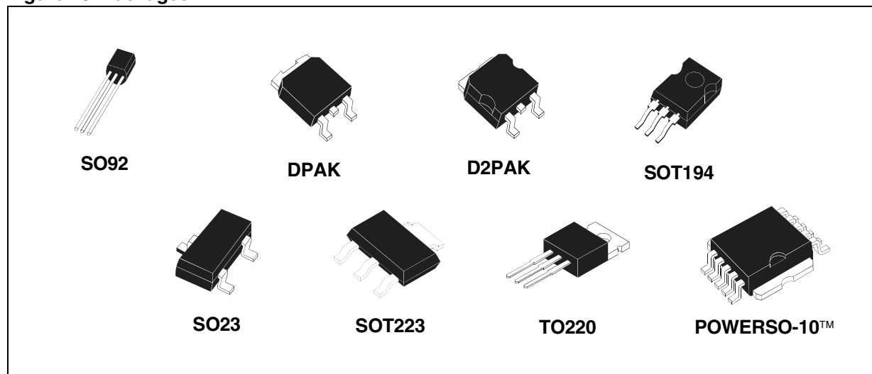
Figure 13. Packages
