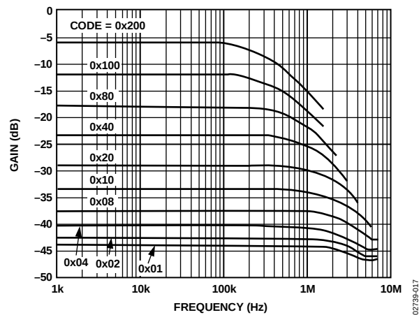
Figure 17. Gain vs. Frequency vs. Code, R_{AB} = 10 k\Omega (Figure 32)
