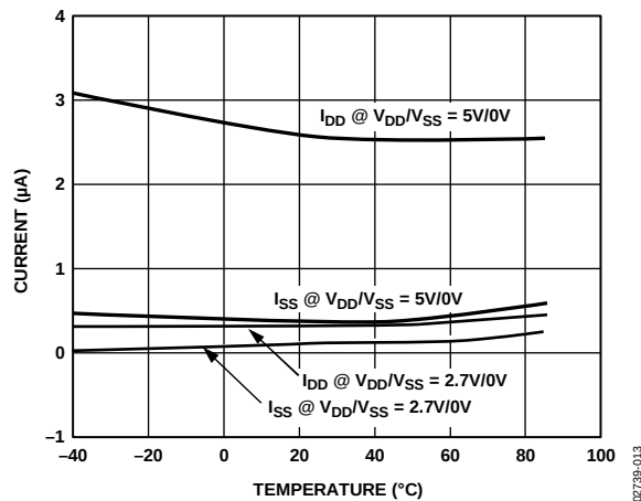
Figure 13. I_{DD} vs. Temperature, R_{AB} = 10 k\Omega
