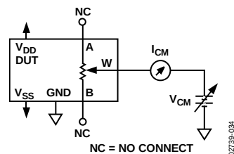
Figure 34. Common-Mode Leakage Current
