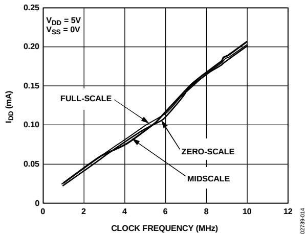
Figure 14. I_{DD} vs. Clock Frequency, R_{AB} = 10 k\Omega
