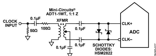
Figure 21. Transformer-Coupled Differential Clock
