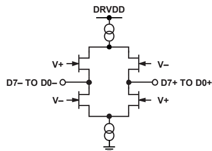
Figure 18. LVDS Output Driver
