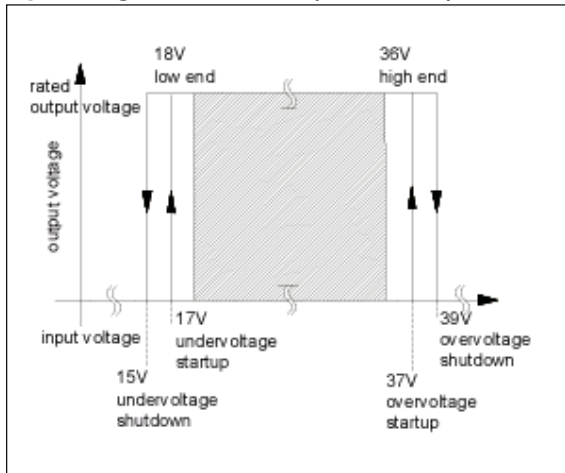
Fig. 1 24V input voltage range (typ.)
