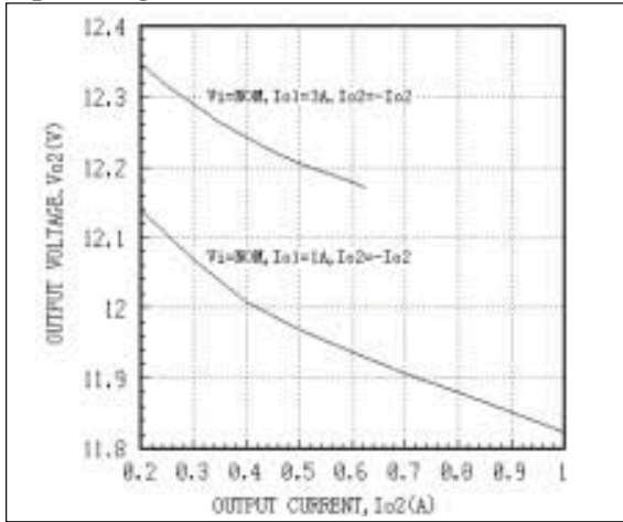
Fig. 25 AEW05ABB48 Load Regulation Curves
