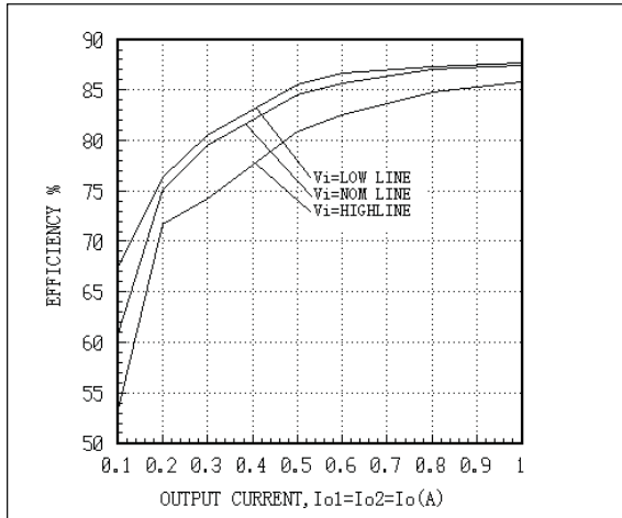
Fig. 9 AEW01CC24 Efficiency Curves
