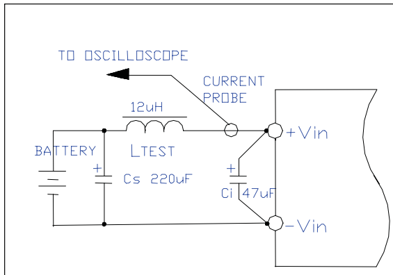
Fig. 3 Reflected noise current testing With 12 \mu H impedance, test point in the input line.
