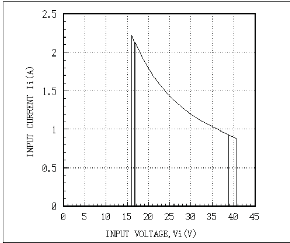
Fig. 13 AEW03AA24 Input Characteristic Curves Tc=25°C
