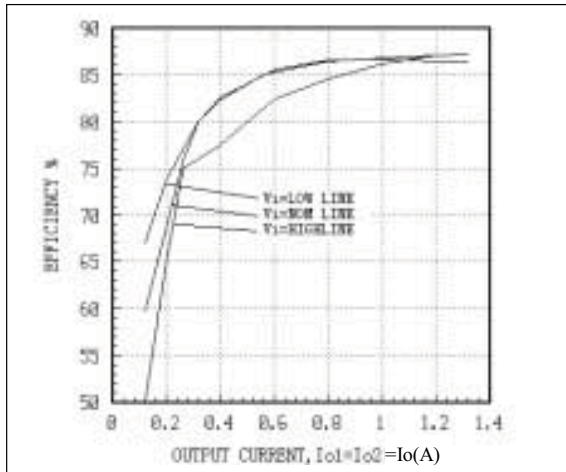
Fig. 11 AEW01BB48 Efficiency Curves
