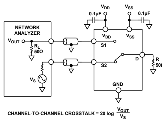
Figure 36. Channel-to-Channel Crosstalk
