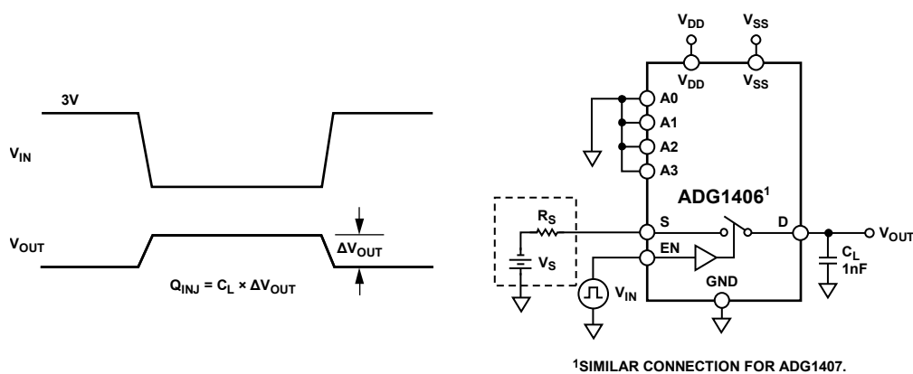
Figure 33. Charge Injection
