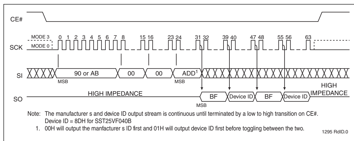
Figure 21: Read-ID Sequence
