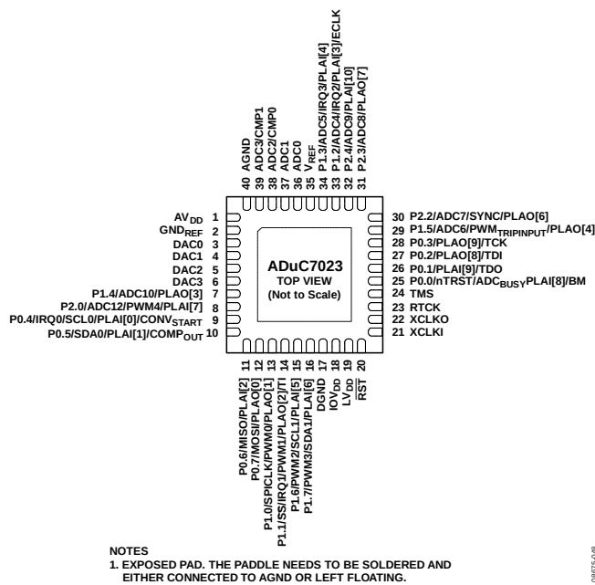
Figure 7. 40-Lead LFCSP Pin Configuration
