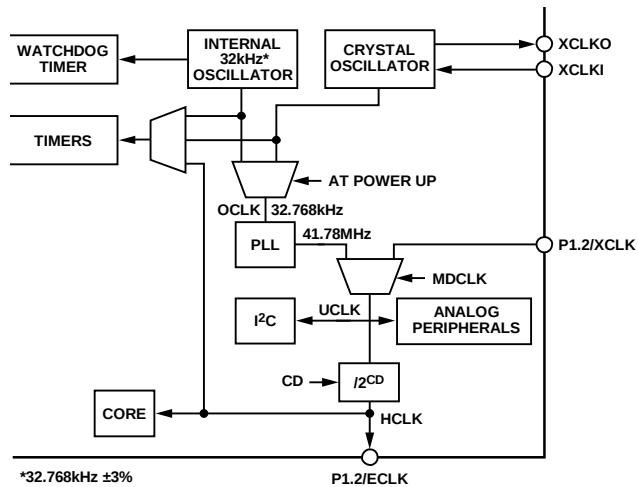
Figure 36. Clocking System
