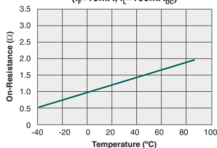
Typical On-Resistance vs. Temperature ( I_F=10\text{mA} , I_L=100\text{mA}_{DC} )
