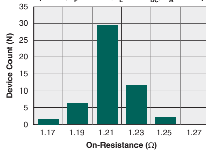
Typical On-Resistance Distribution (N=50, I_F=10\text{mA} , I_L=0.7\text{A}_{DC} , T_A=25^\circ\text{C} )
