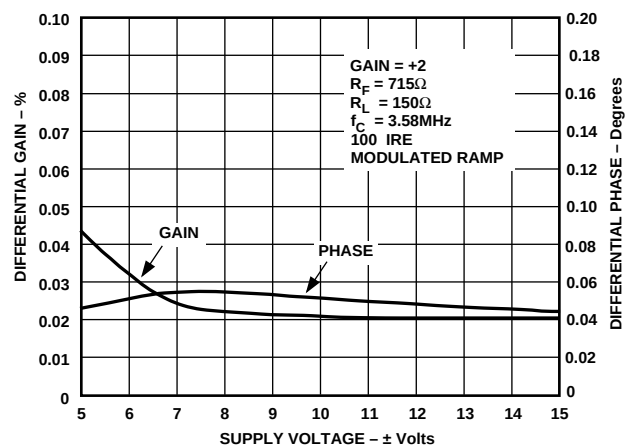
Figure 49. Differential Gain and Phase vs. Supply Voltage
