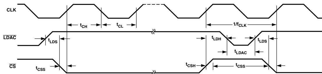
Figure 3. Continuous Clock Timing Diagram
