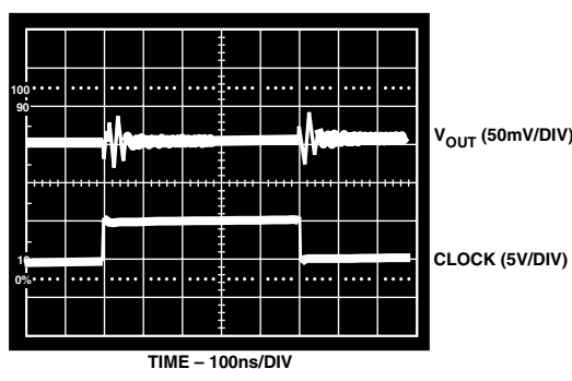
TPC 11. AD7398 Digital Feedthrough
