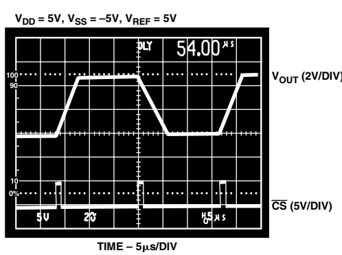
TPC 12. AD7398 Large Signal Settling Time
