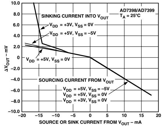
TPC 8. \Delta V_{OUT} vs. Load Current
