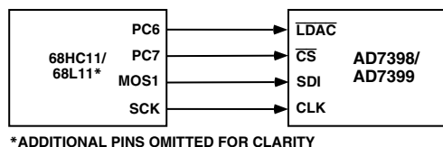
Figure 9. 68HC11/68L11 to AD7398/AD7399 Interface
