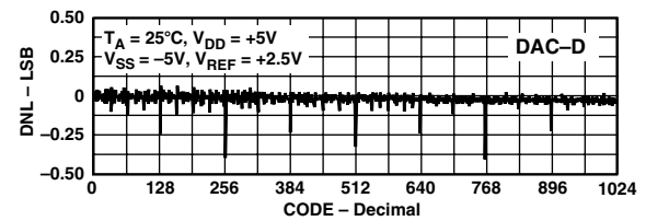
TPC 3. AD7398 DNL vs. Code ( T_A = 25^\circ\text{C} )
