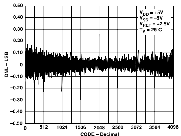
Figure 1. AD7398 DNL vs. Code ( T_A = 25^{\circ}\text{C} )
