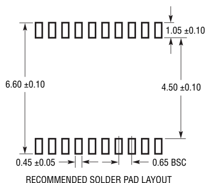
F Package 20-Lead Plastic TSSOP (4.4mm) (Reference LTC DWG # 05-08-1650)
