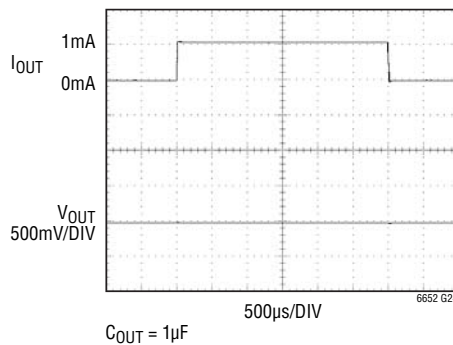
1.25V Sinking Current with Output Capacitor
