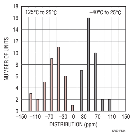
Figure 13b. LS8 Hysteresis Plot -40^{\circ}\text{C} to 125^{\circ}\text{C}
