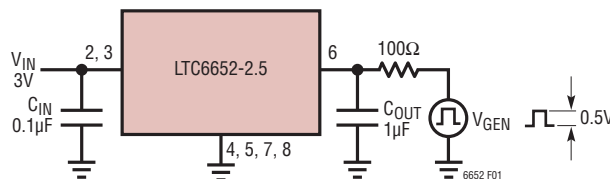
Figure 1. Transient Load Test Circuit
