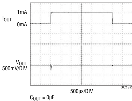
1.25V Sinking Current Without Output Capacitor
