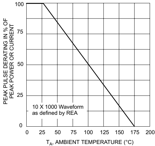
Fig. 4, Derating Curve
