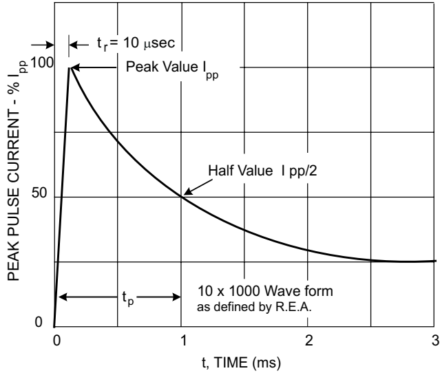
Fig. 1, Pulse Waveform
