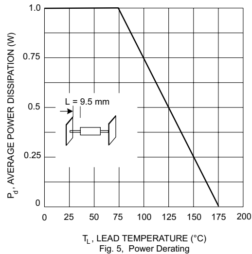
Fig. 5, Power Derating
