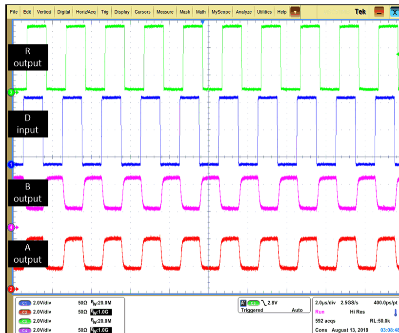
Figure 31. Waveforms at 1 Mbps Operation, Clock Data Pattern
