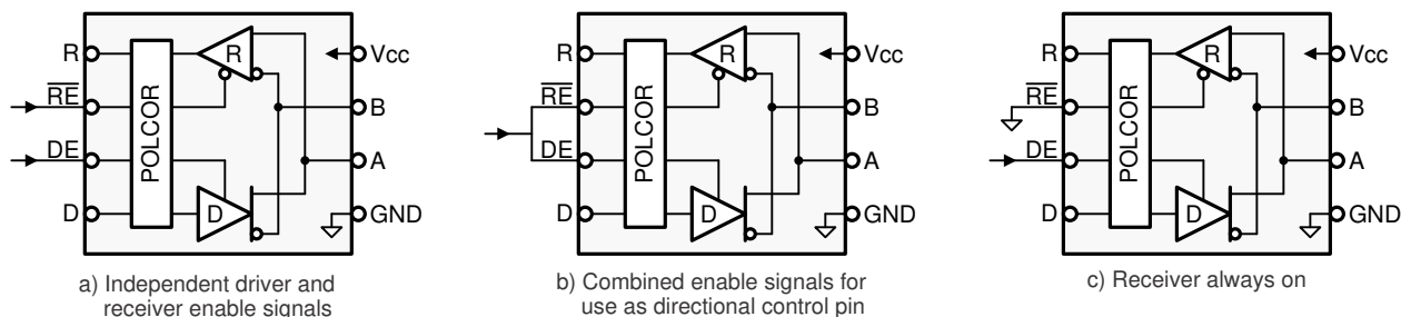
Figure 22. Transceiver Configurations
