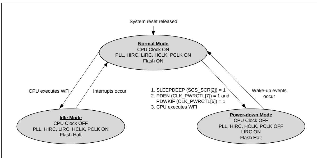
Figure 6.2-7 Power Mode State Machine
