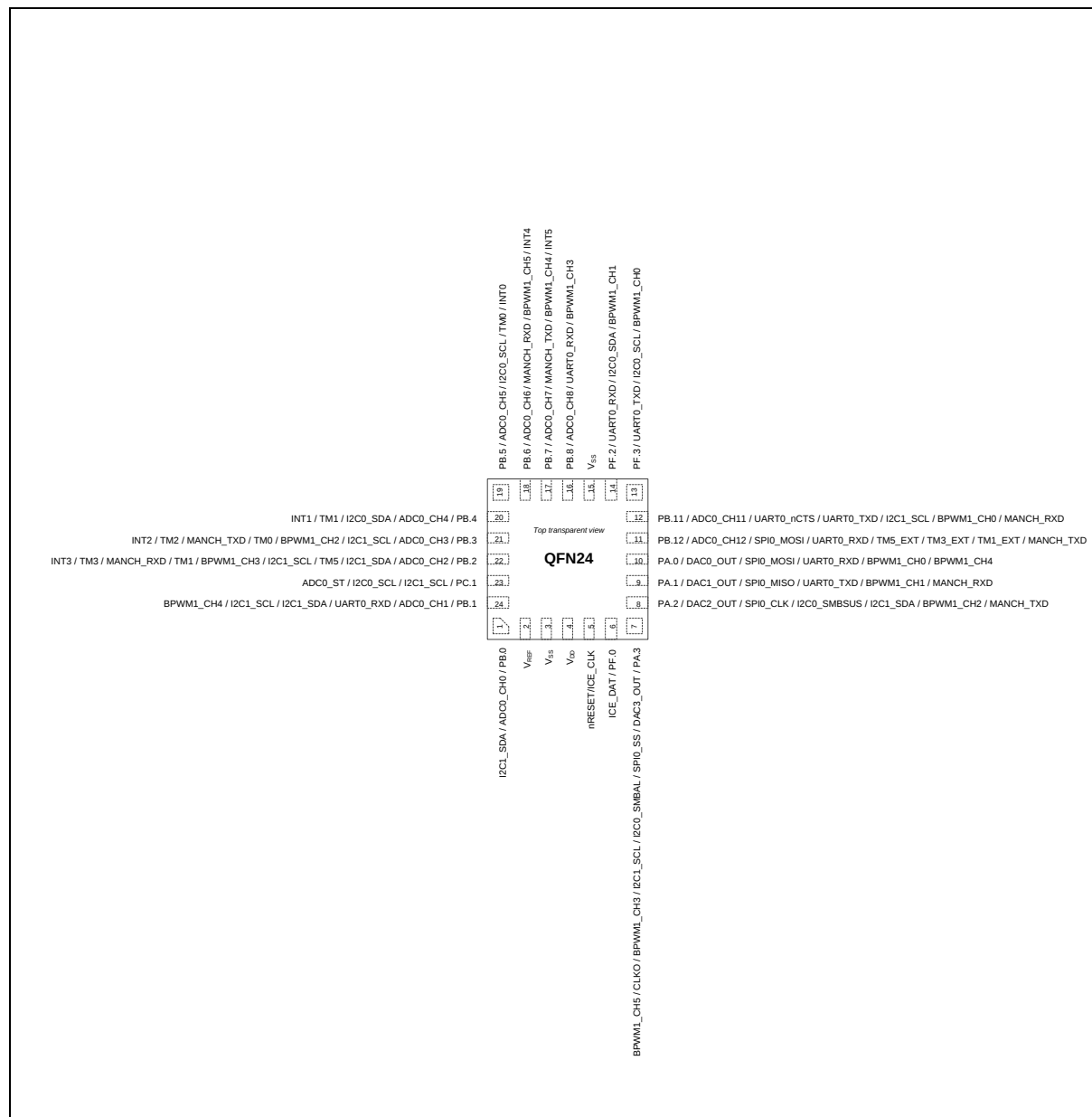
Figure 4.1-5 M031G Series QFN 24-pin Multi-function Pin Diagram
