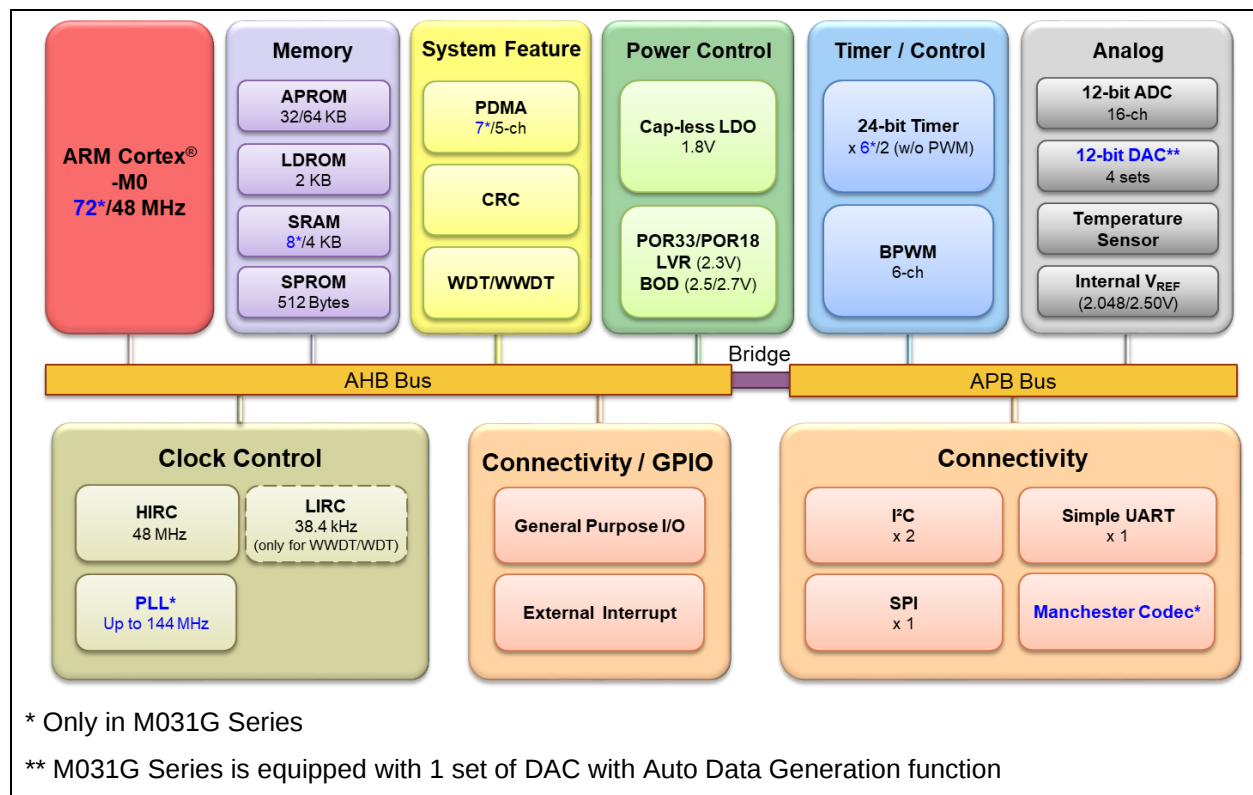
Figure 5-1 NuMicro M030G/M031G Block Diagram
