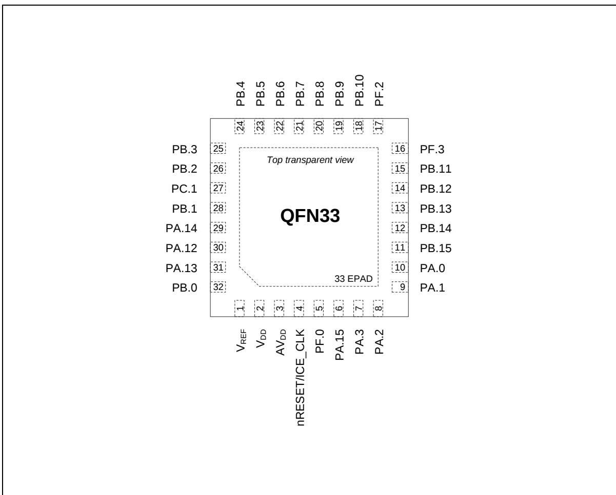
Figure 4.1-2 M030G/M031G Series QFN 33-pin Diagram
