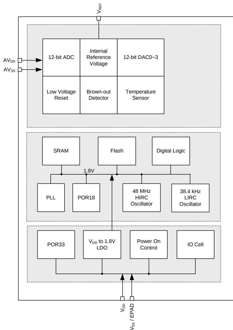
Figure 6.2-6 NuMicro® M030G/M031G Power Distribution Diagram
