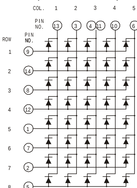
LM23058D (Common Anode Row)
