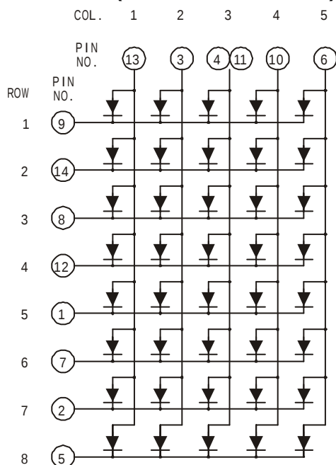
LM23058C (Common Cathode Row)
