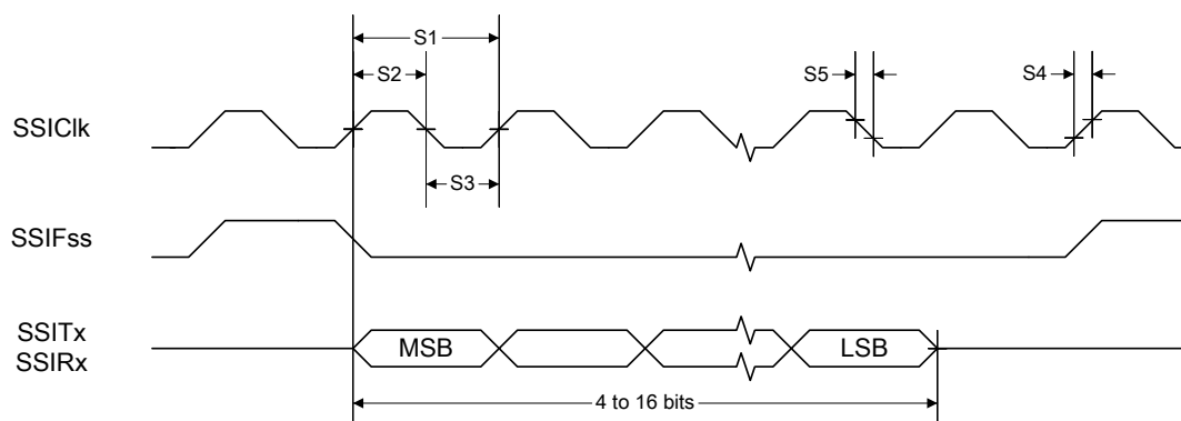
图 23-20. SSI Timing for TI Frame Format (FRF=01), Single Transfer Timing Measurement
