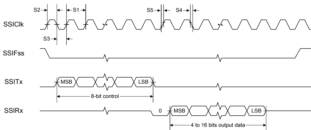
图 23-21. SSI Timing for MICROWIRE Frame Format (FRF=10), Single Transfer
