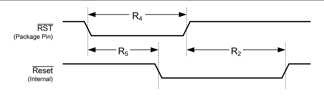
图 23-12. Software Reset Timing
