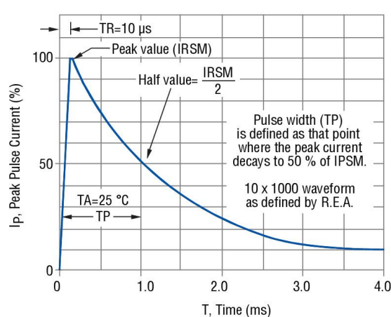
Figure 4- Pulse Waveform
